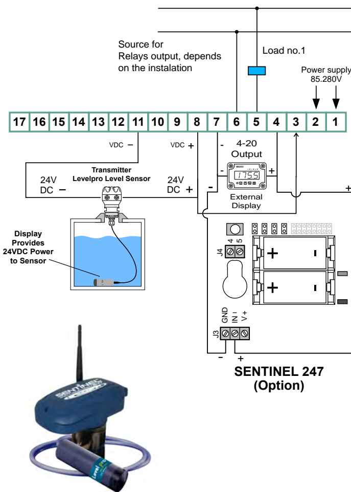
100 Series with Sentinel Telemetry Device
