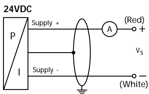
2-wire-system (current)
