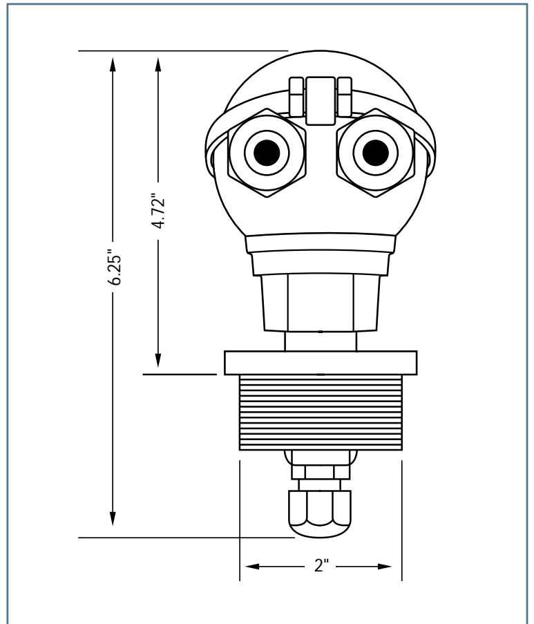
Easy Access Clamshell Design 4-Pole Electrical Connection
