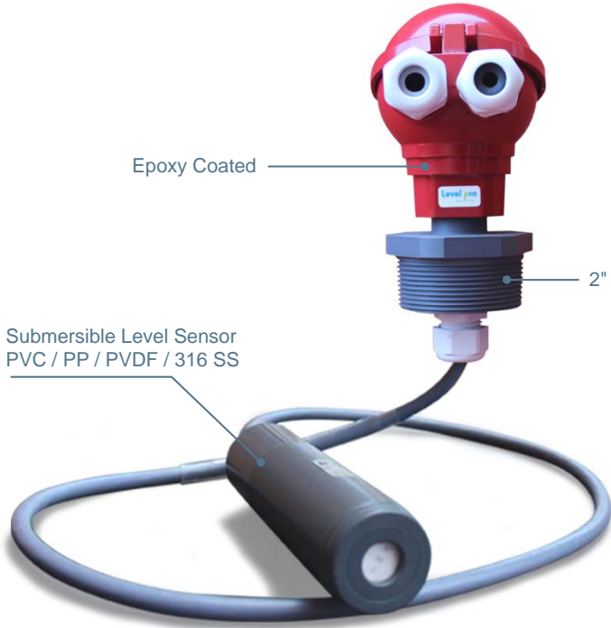
Easy Access Clamshell Design 4-Pole Electrical Connection
