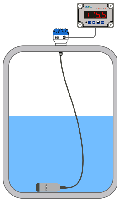
Connect Sensor to Display
